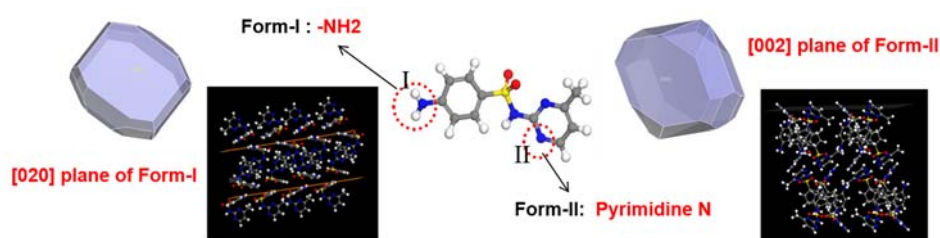
Fig. 1. Molecular simulation of polymorphic shapes of sulfamerazine in a water/acetonitrile solvent.
